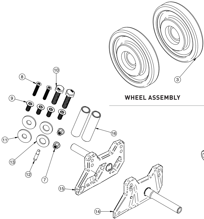
AC6 ADAPTER ASSEMBLY
